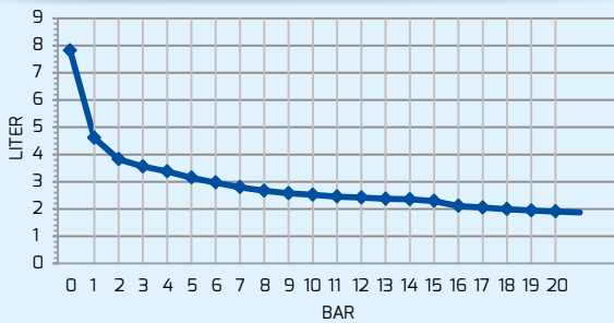
LARA 2L/20B
