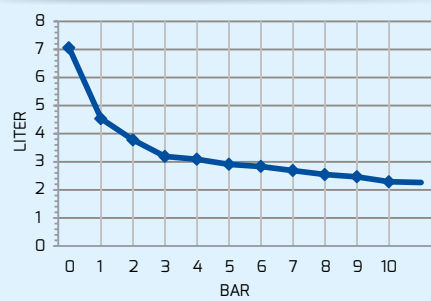
LARA 2L/10B
